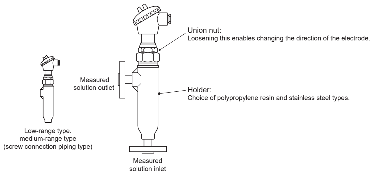
Figure 2.1 Conductivity Detector
