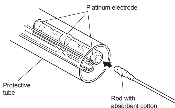
Figure 5.1 Cleaning an Electrode with a 5 \text{ cm}^{-1} Cell Constant
