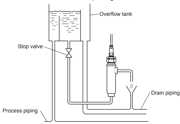
Figure 3.7 Example of Sampling Piping with Bubble Removal Function
