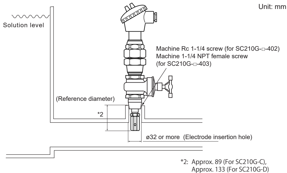
Figure 3.2 Procedure for Electrode Insertion Hole Processing for the Direct Insertion Type Detector with Gate Valve
